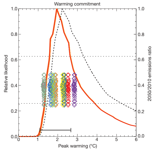
Figure 3 | Warming commitment for selected scenarios shown in Fig. 1a. Red and orange curves (superimposed) show likelihood profiles for cumulative warming commitment (CWC) under 49 scenarios with total emissions within 1% of 1 Tt C estimated with the simple climate-carbon-cycle model; dotted black curve shows likelihood profile for peak warming under '490 p.p.m. stabilization' scenario. Horizontal dotted lines show warming thresholds for the 17–83% and 5–95% confidence intervals 19 . The horizontal location of coloured symbols shows corresponding 1 Tt C CWCs predicted by HadSCCM1 fitted to the ESMs in the C 4 MIP ensemble. The vertical location and right-hand axis shows fractional decrease in emissions from 2010 to 2050 for each of the 49 emissions scenarios. Solid error bar shows 5–95% Bayesian posterior probability interval (1.1–2.7 °C) for 1 Tt C CWC based on an independent model and approach 20 .
